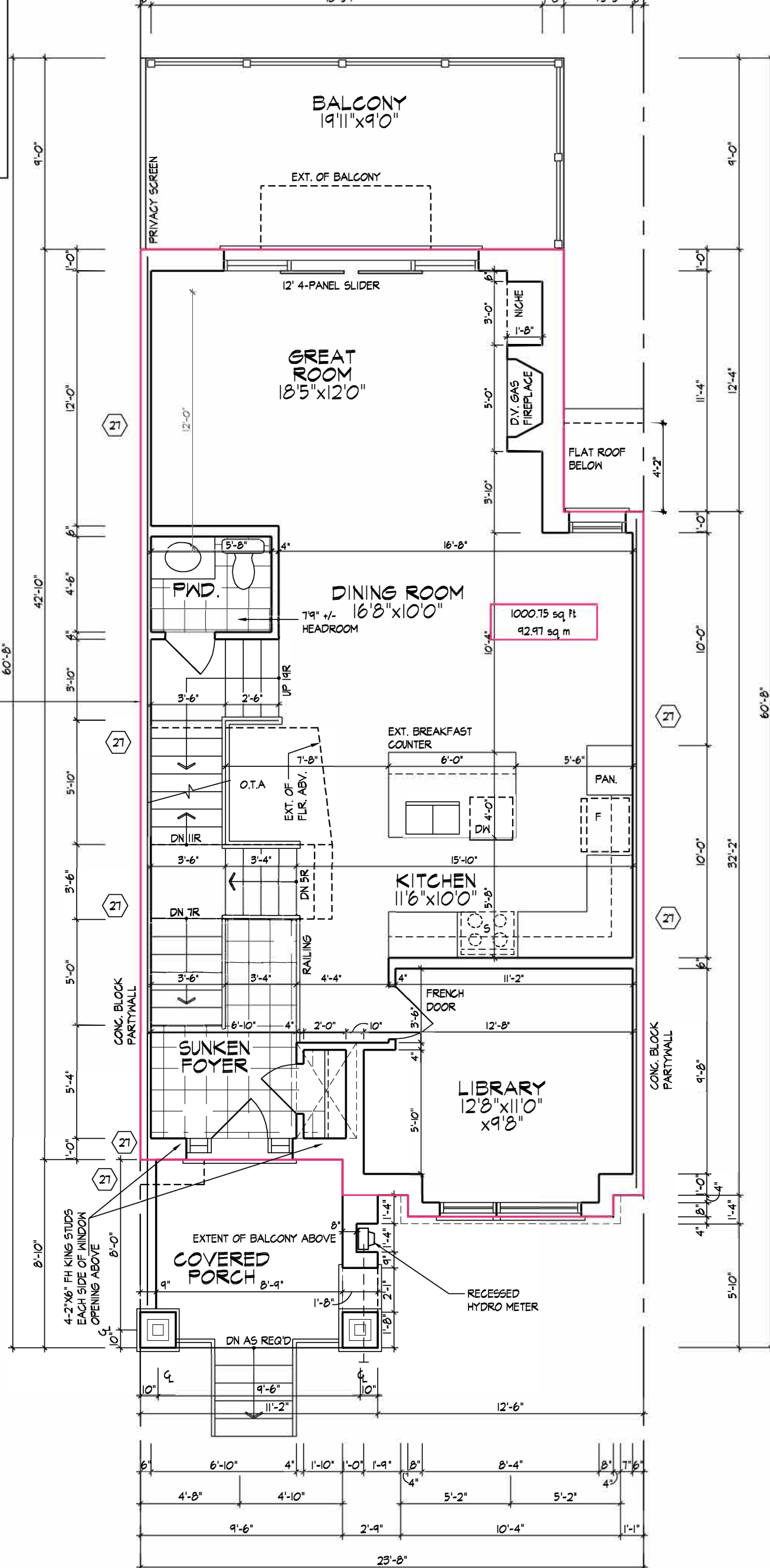
MAIN FLOOR PLAN, EL. 'B' - UNIT 2 BLK 13
