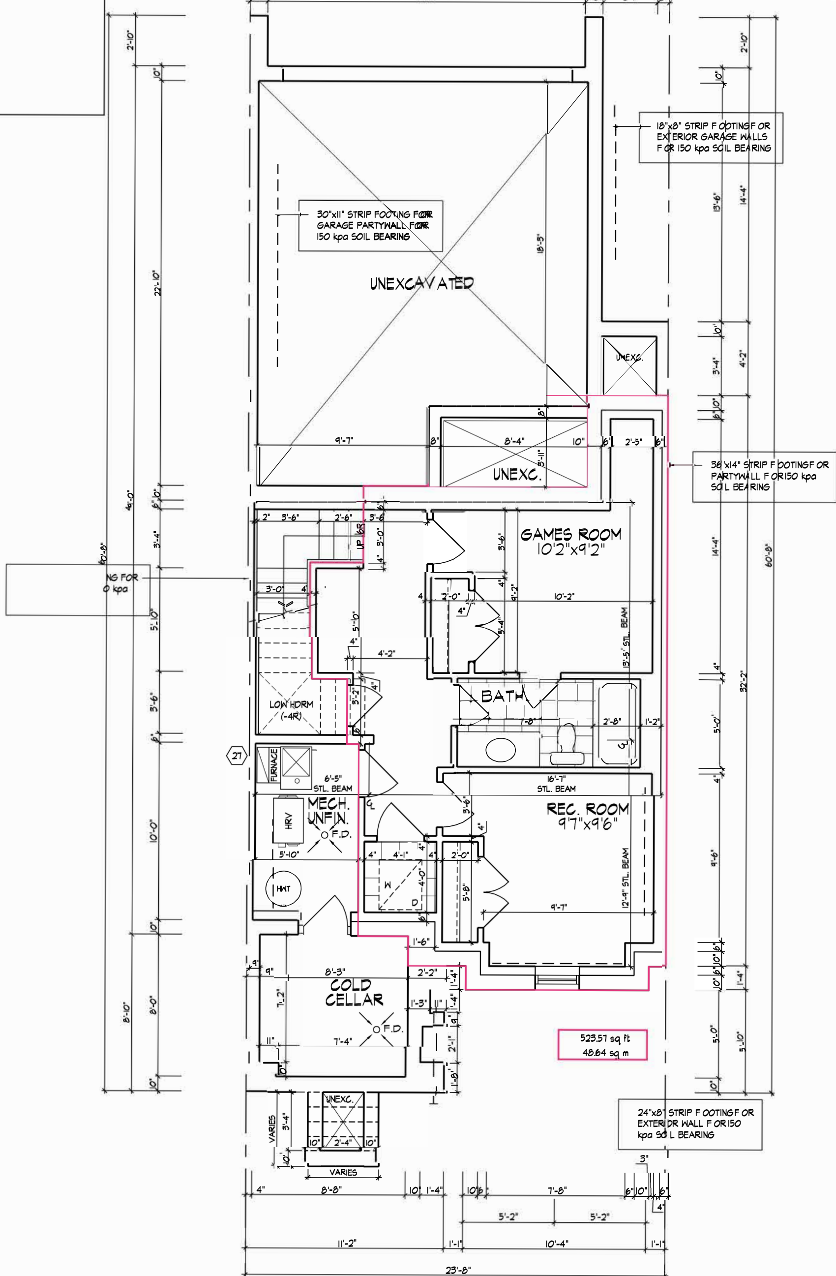
FIN. BASEMENT PLAN, EL. 'B' - UNIT 2 BLK 13
